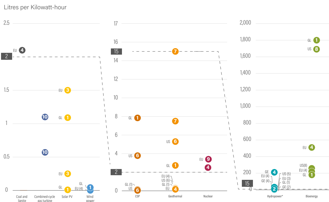
FIGURE 8. Estimated Water Footprint of Different Energy Generation Technologies
